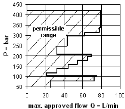
Permissible Operating Range
